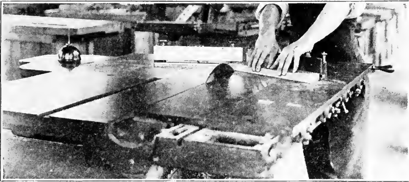
FIG. 163. SAWING SIMPLE MITERS.
